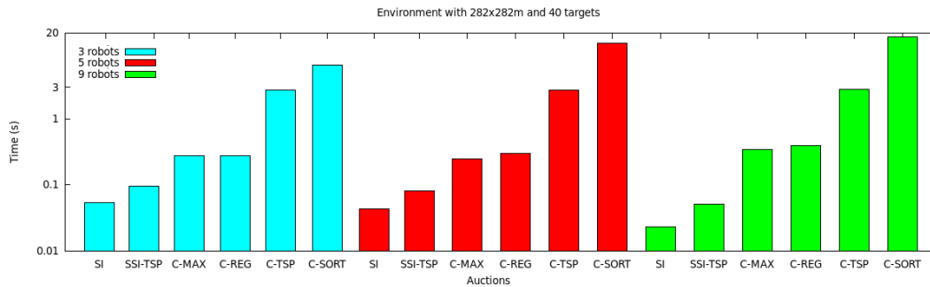
Fig. 7. Time consumed by the auctions to compute the allocations in scenarios with 40 targets non-uniformly distributed.
