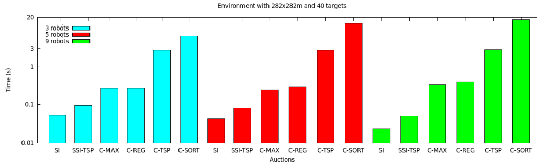
Fig. 6. Time consumed by the auctions to compute the allocations in scenarios with 40 targets uniformly distributed.
