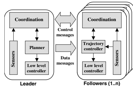
Figure 1: Architecture for tightly coupled cooperation
