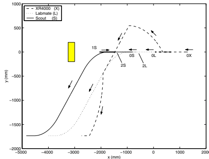
Figure 10: Experiment 3 - the Scout requests the leadership (1S) and returns it (2S) to the Labmate
