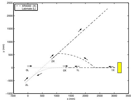
Figure 6: Experiment 1 - the XR4000 resigns the leadership (1X) and receives it back (2X)
