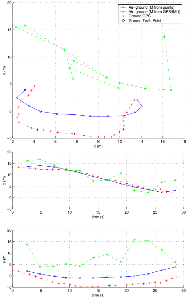
Fig. 9. Estimated robot trajectory.
