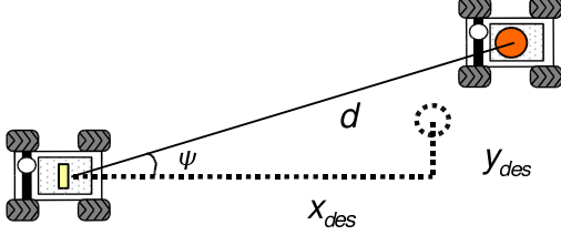
Fig. 3. Leader-follower controller.
