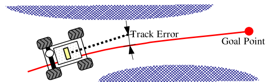
Fig. 2. Path-follower controller.
