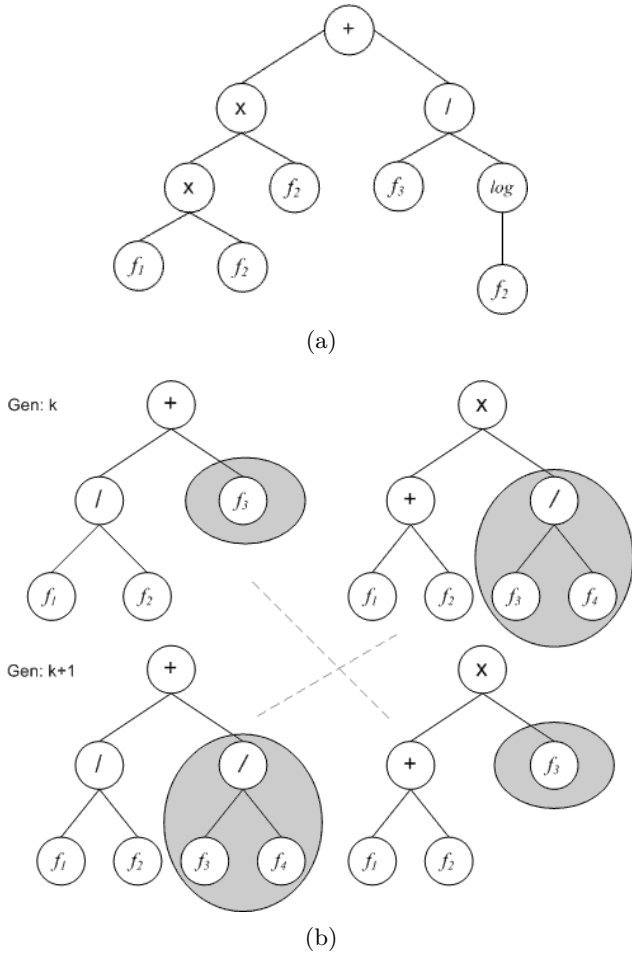
Figure 2: CBIR-GP individuals (a) are similarity functions (from potentially different descriptors) combined by arithmetic operators; the Genetic Programming scheme combines “material” from different individuals in the population from one generation to another using, for example, a crossover operations (b).
