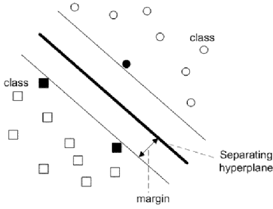
Figure 1: The SVM classifier finds the hyperplane which separates the two classes (here exemplified by squares and circles) with the widest possible margin.
