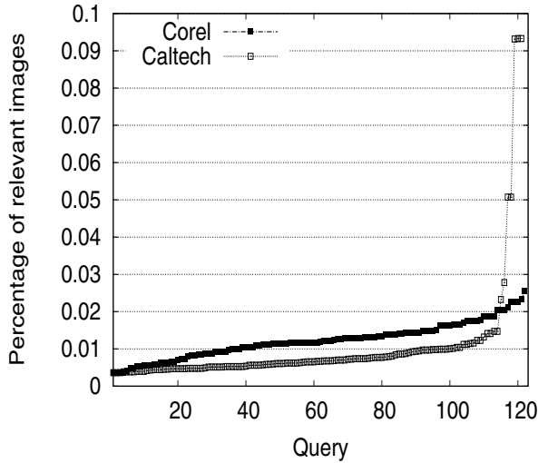
Figure 3: Distribution of relevant images, indicating the expected abundance/scarsity of correct answers for each query. This has an impact on the degree of difficulty of the retrieval task (this distribution indicates that the Caltech database is more challenging).
