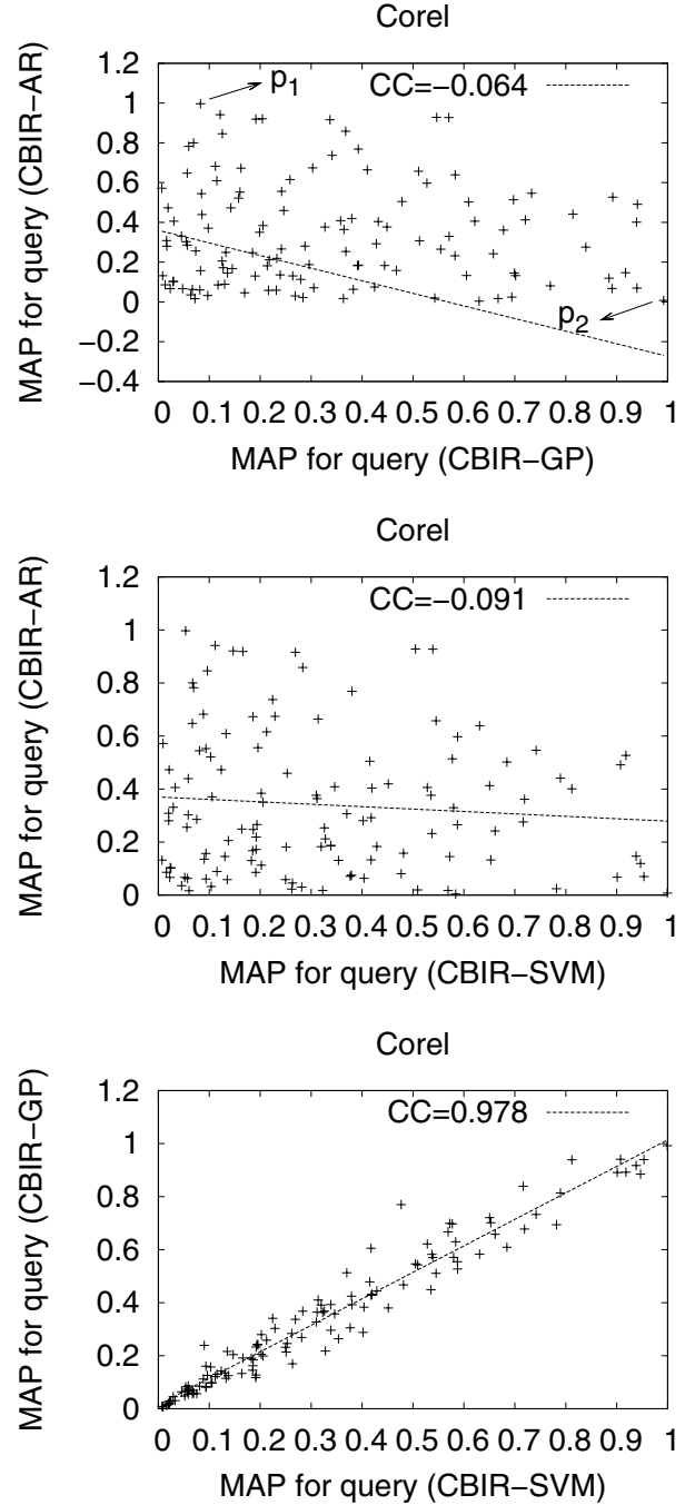
Figure 4: Each graph shows a scatter plot of the MAP values obtained for each query on two different schemes. On top: CBIR-AR x CBIR-GP; on middle CBIR-AR x CBIR-SVM; on bottom CBIR-GP x CBIR-SVM. The correlation coefficient (CC) is shown inside each graph.
