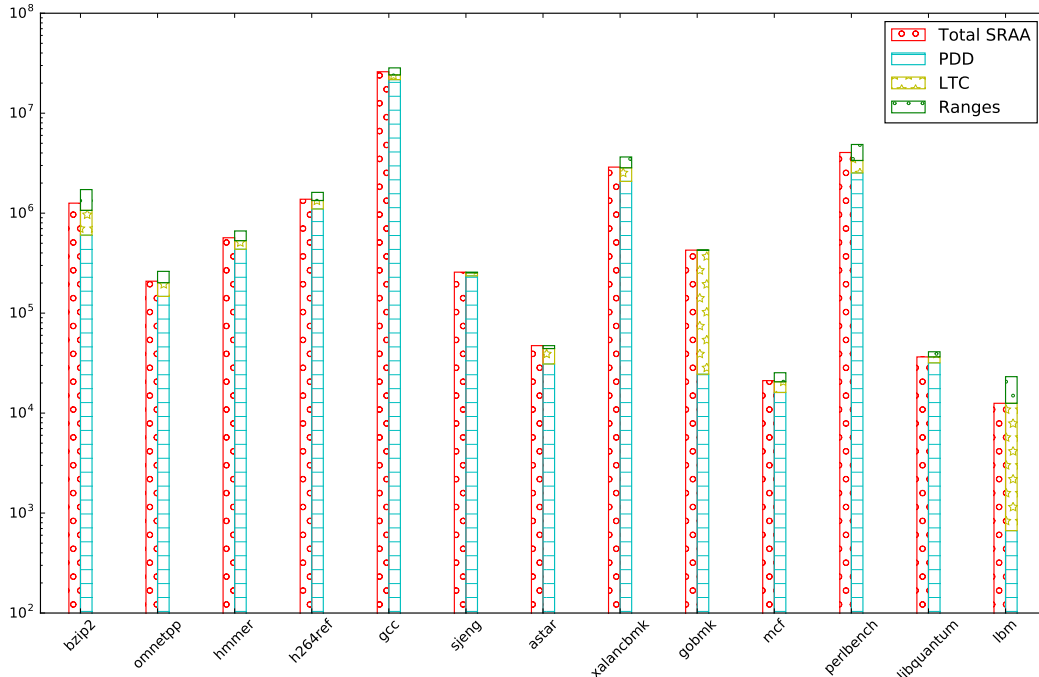
Figure 21: How three tests in SRAA separately compete to disambiguate pairs of pointers. The Y-axis denotes the number of disambiguated pairs of pointers.
