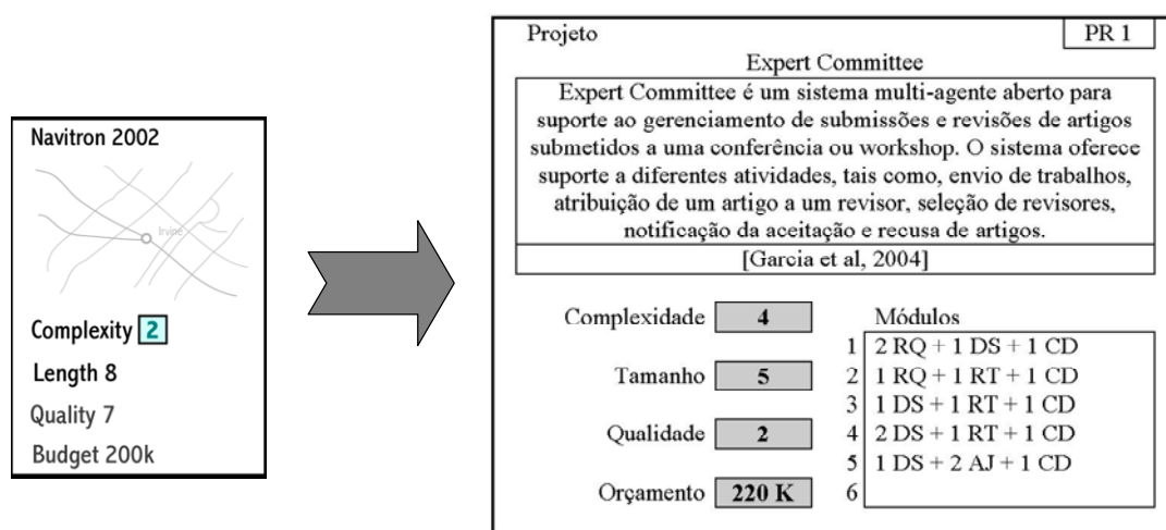
(a) PnP
