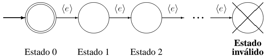
Figura 5.19: O problema de state build-up .
