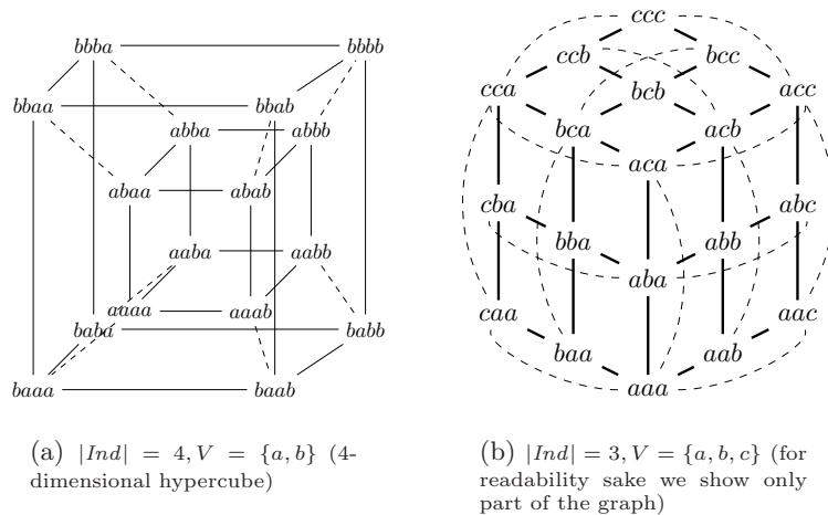
Fig. 3. Some (V^{Ind}, \sim) graphs
