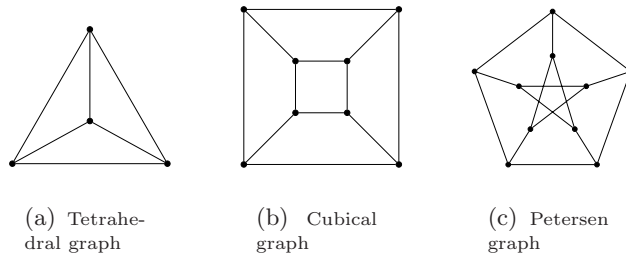
Fig. 1. Some distance-regular graphs with degree 3.
