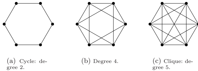
Fig. 2. Some VT^+ graphs
