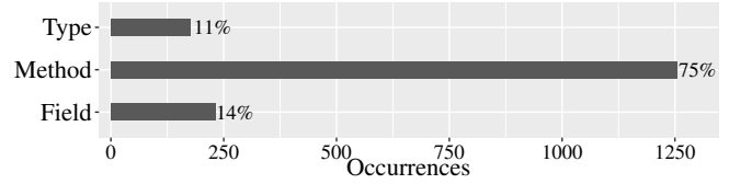
(a) PHILJAY/MPANDROIDCHART
