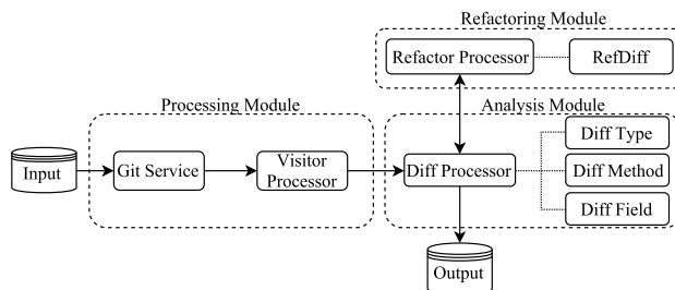
Fig. 1. APIDiff Architecture
