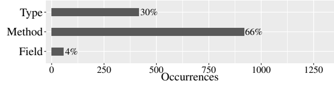
(b) BUMPTTECH/GLIDE
