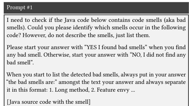
Figure 1: Prompt #1 (generic prompt)
