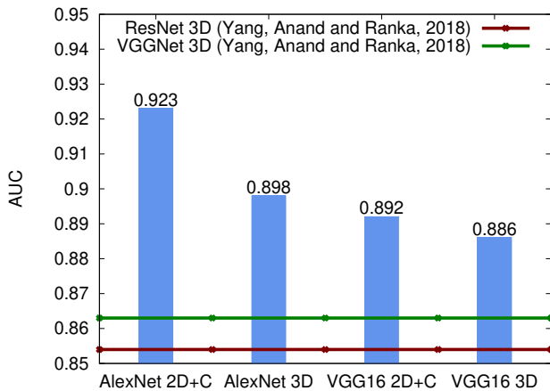
Fig. 2: Classification performance of different models.
