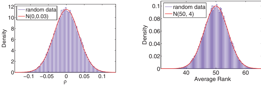
(a) Spearman \bar{\rho} distribution. The distribution was fitted to a normal distribution N_{\rho}(0, 0.03) .
